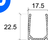
BOTTOM U-CHANNEL
