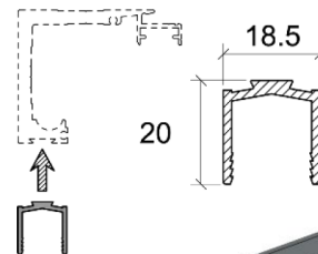
DOVETAILED U-CHANNEL
